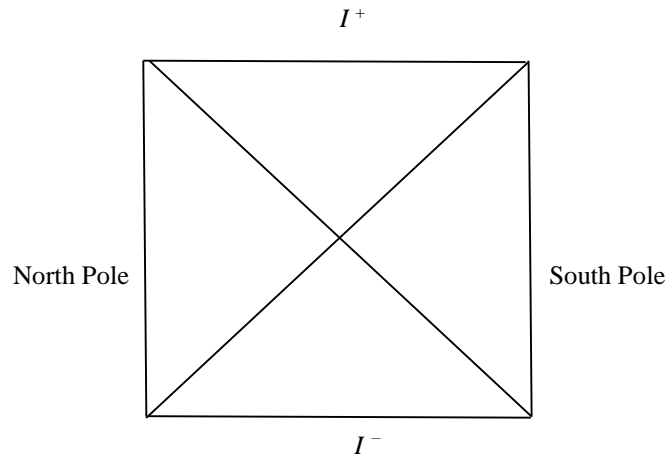
Figure 1. Penrose diagram of de Sitter space.
